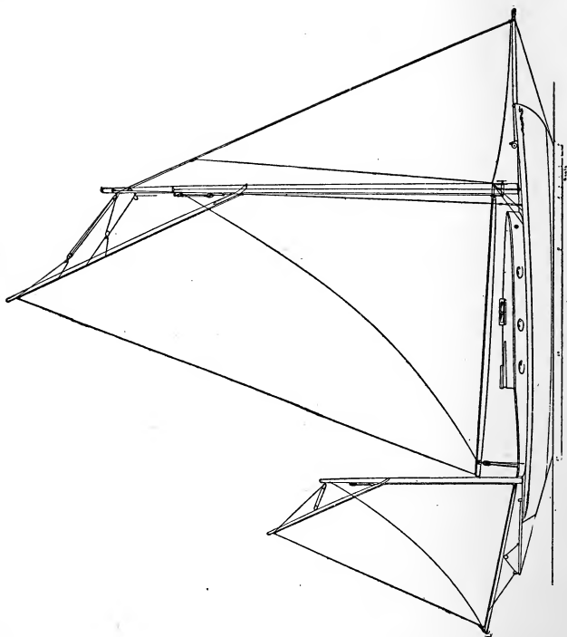
RIG AND SAIL PLAN OF A MODERN YAWL.
